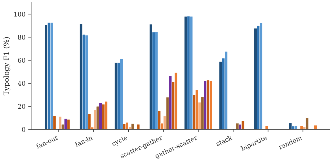
Per-Class Typology F1: ML vs LLMs — HI-Small
