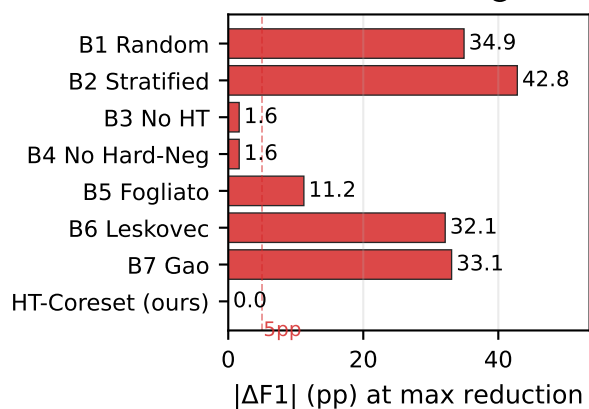
LI-Small: baselines @ 611x
