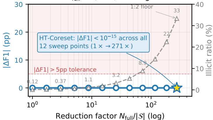
HI-Small: N_{\text{full}} = 1,015,669 edges
