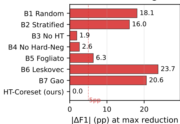
HI-Small: baselines @ 271x
