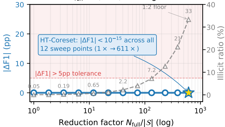
LI-Small: N_{\text{full}} = 1,384,810 edges
