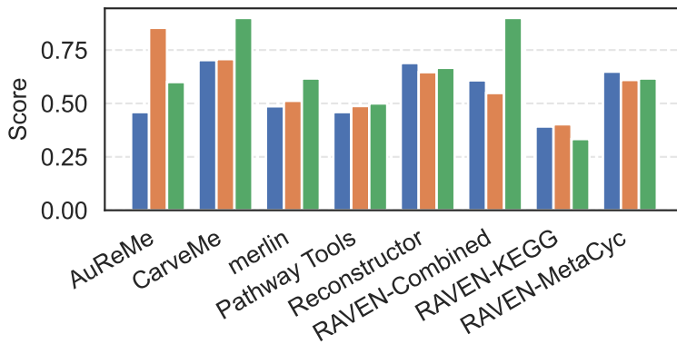
Biomass score
