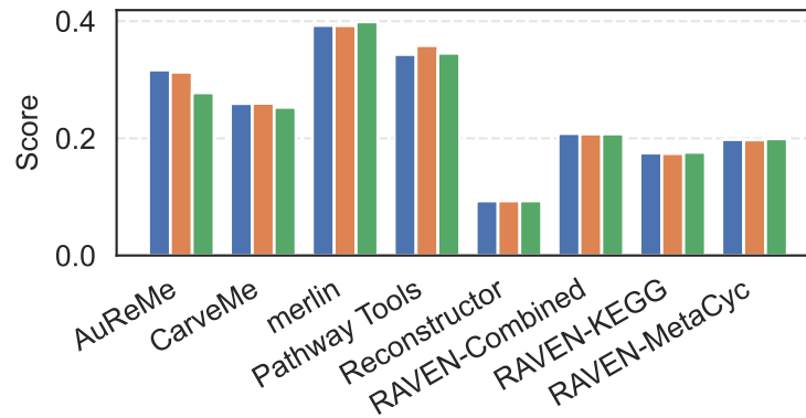
Annotation score
