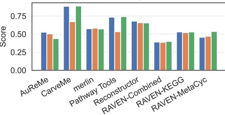
Consistency score
