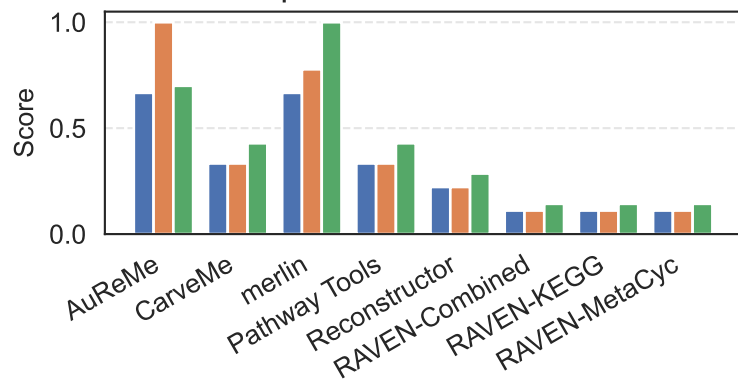
Consistency score
