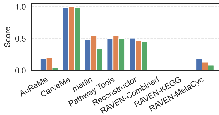
Annotation score
