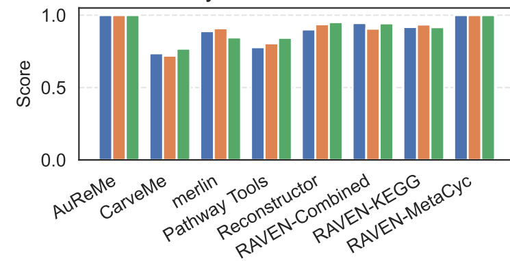
Biomass score
