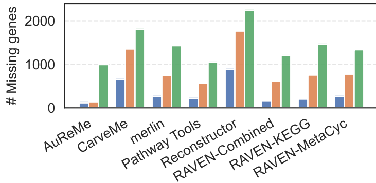
Missing genes
