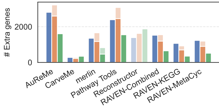
Extra genes
