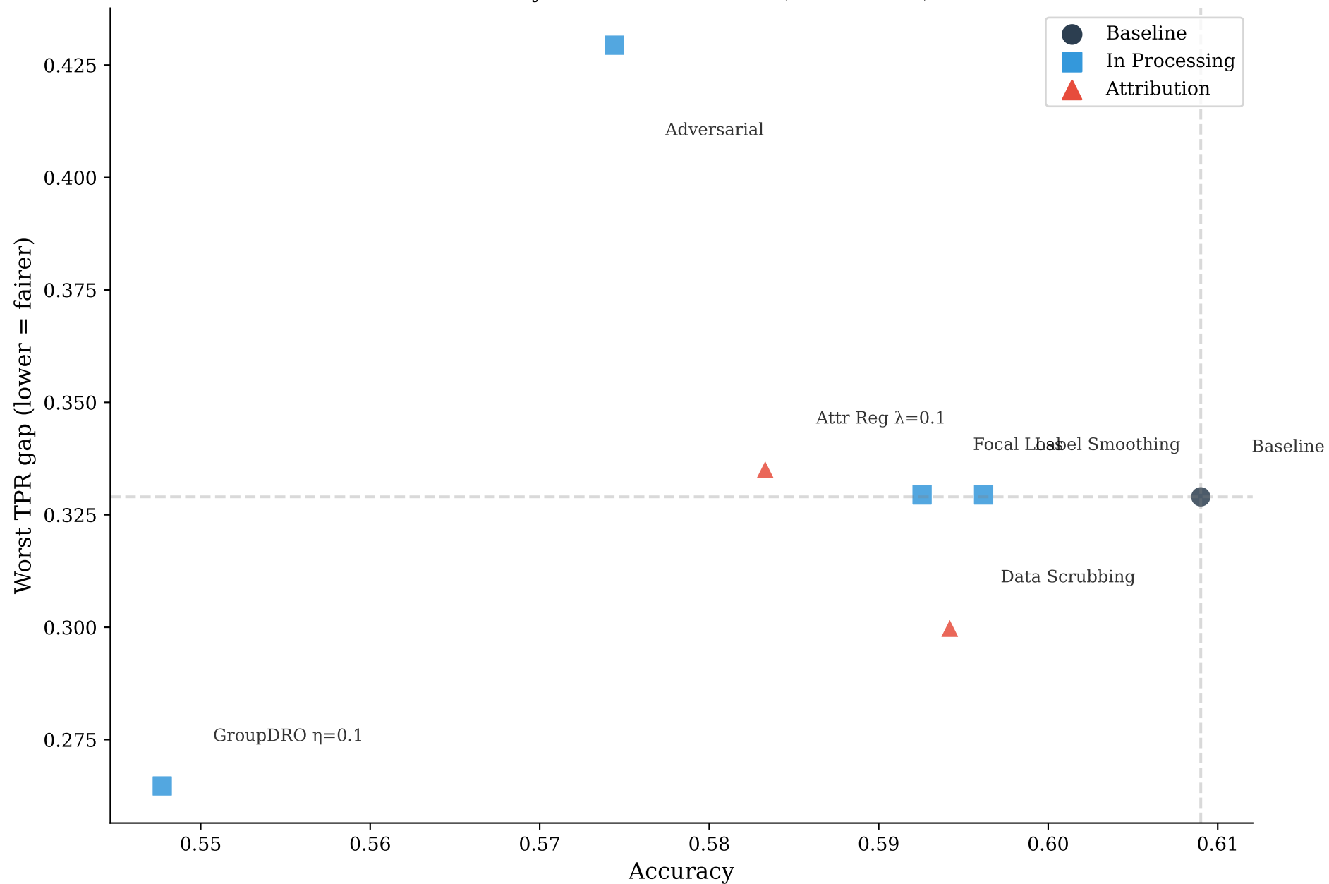
Accuracy-fairness trade-off (main track)
