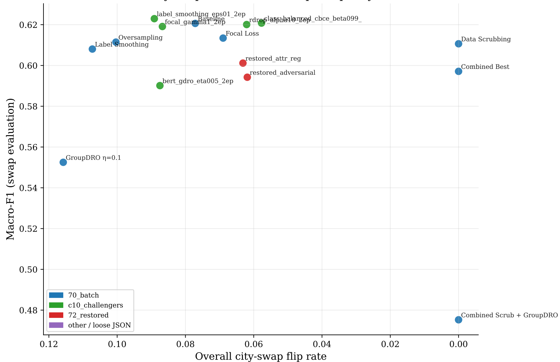
City-swap robustness vs swap-set quality
