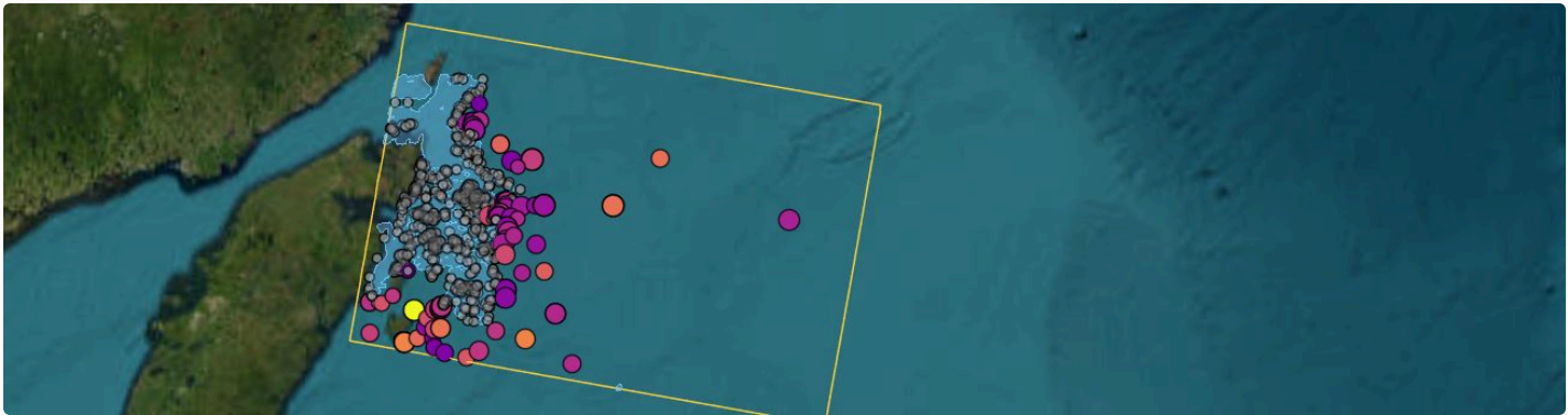
The viewer, 2 May 2025: scene footprint (yellow), pack ice (blue), candidates coloured by radar contrast, likely ice floes in grey.
