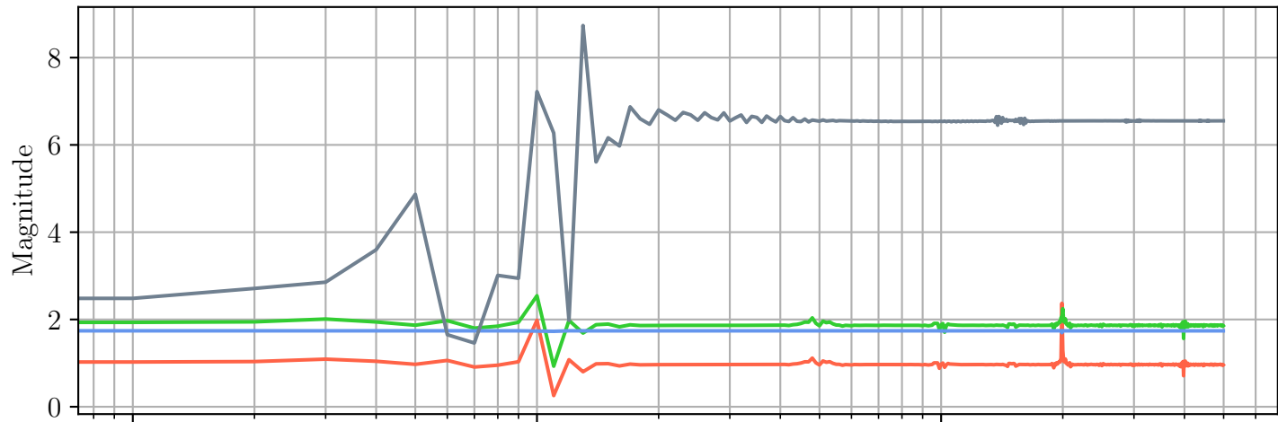
Impedance Bode Plot
