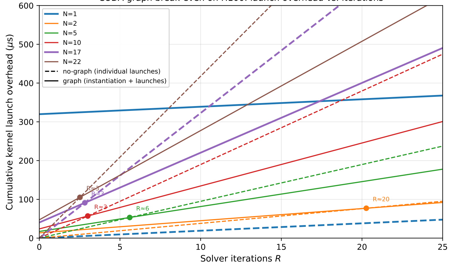
CUDA graph break-even on H100: launch overhead vs. iterations
