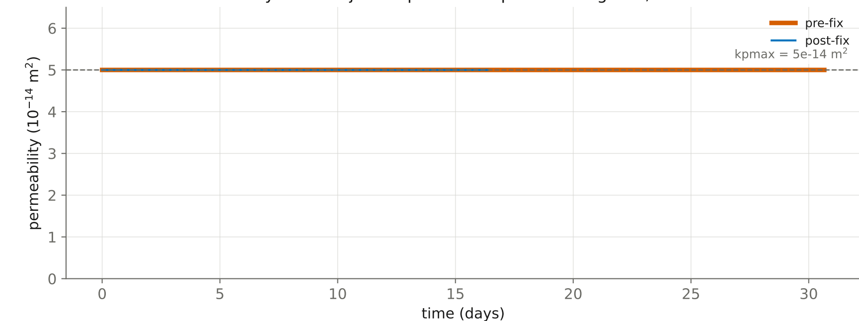
Permeability at the injector: pinned at k pmax throughout, in both runs
