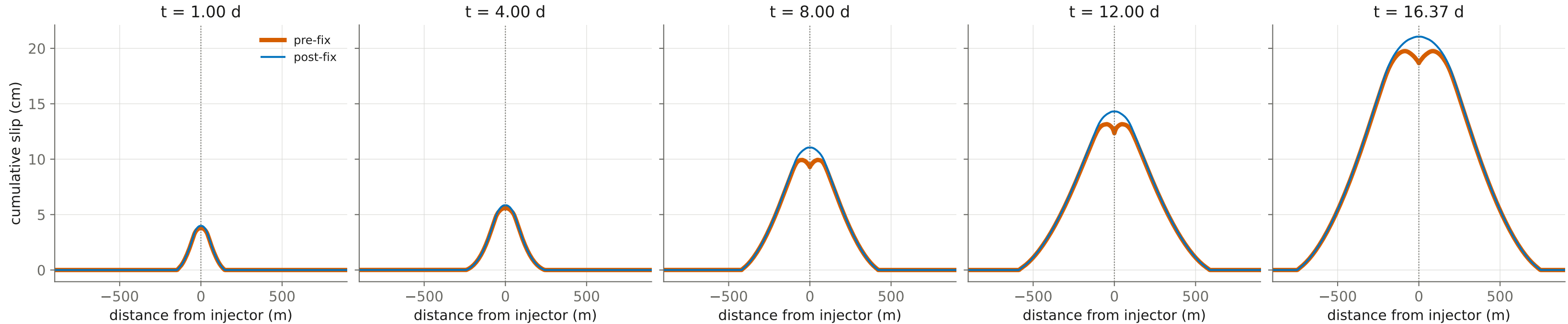
Slip through the injector -- the pre-fix cusp deepens with time
