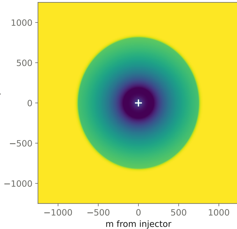
pre-fix (sigma, MPa)
