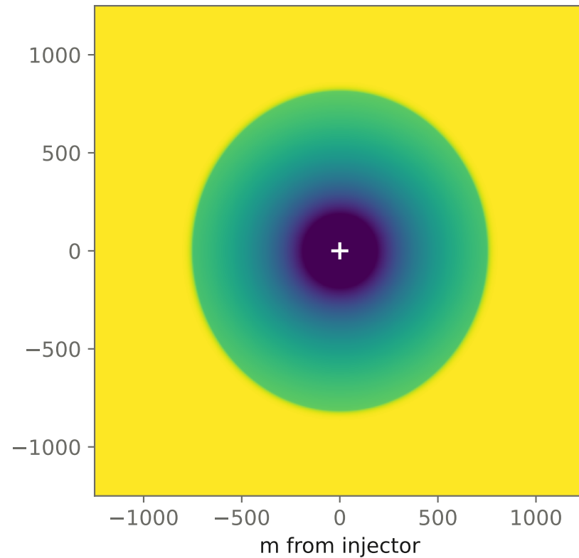
sigma at t = 16.37 d post-fix (sigma, MPa)
