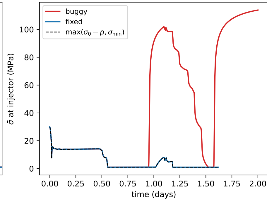
effective normal stress
