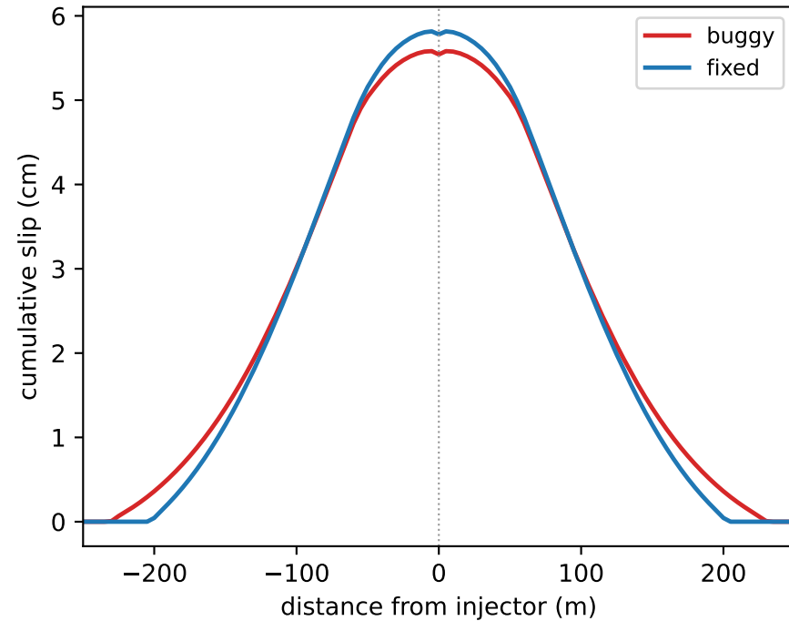
final slip through the injector
