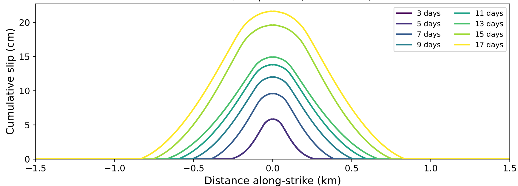
Simulation, cusp fixed (run 632895)
