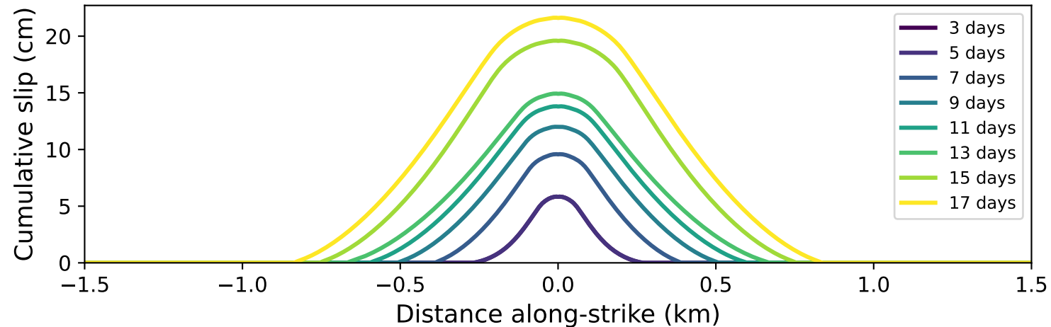
Simulation, cusp fixed (Job 632895)
