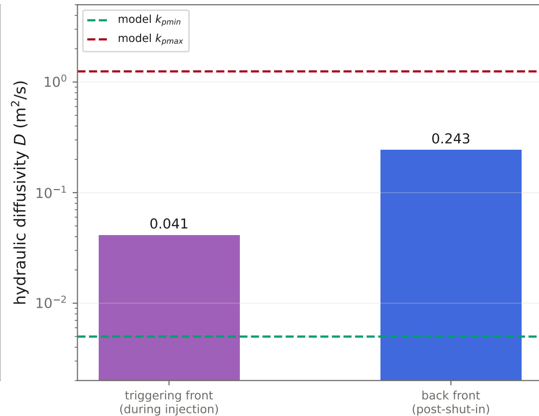
C. Two MODEL-FREE diffusivities. Ratio 5.9x = the permeability enhancement (the decks assume 250x)
