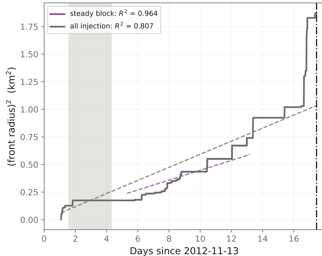
B. The \sqrt{t} test — straight lines mean R \propto \sqrt{t} . A STAIRCASE: each step is a rate increase, so \sqrt{t} is a trend, not the mechanism
