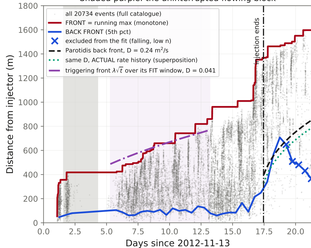
A. Front (monotone) and back front. Shaded purple: the uninterrupted flowing block
