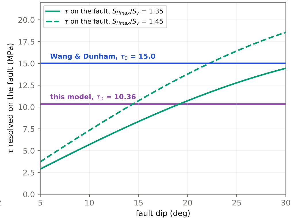
C. Both stress states are admissible. Holl & Barton cannot distinguish them.
