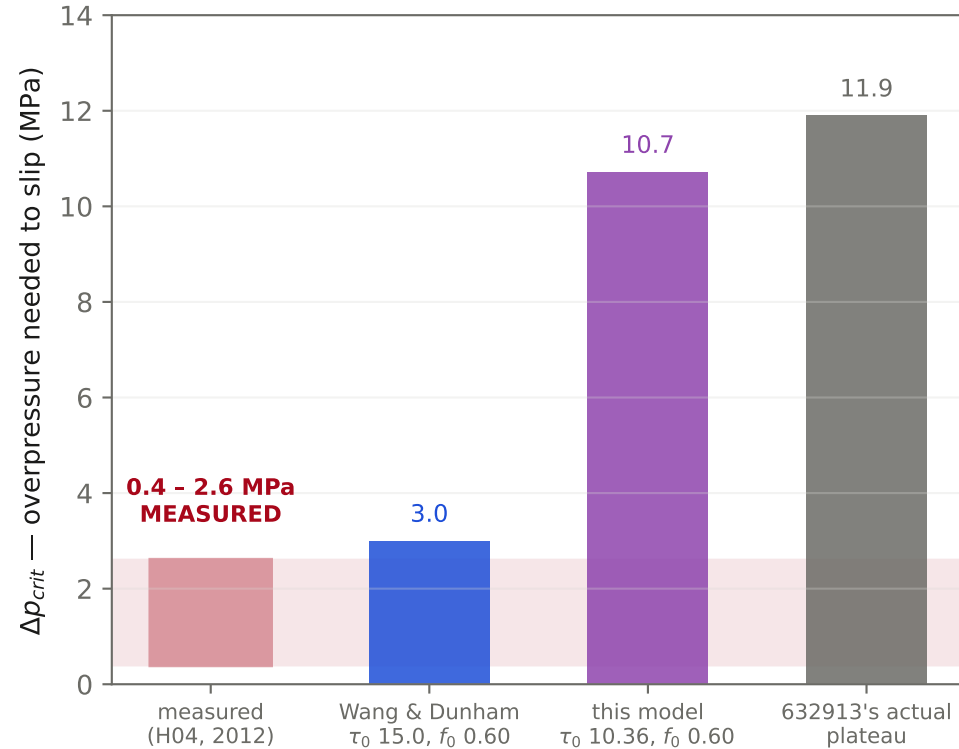
A. The fault slipped at \sim 1 MPa. The model needs \sim 11 .
