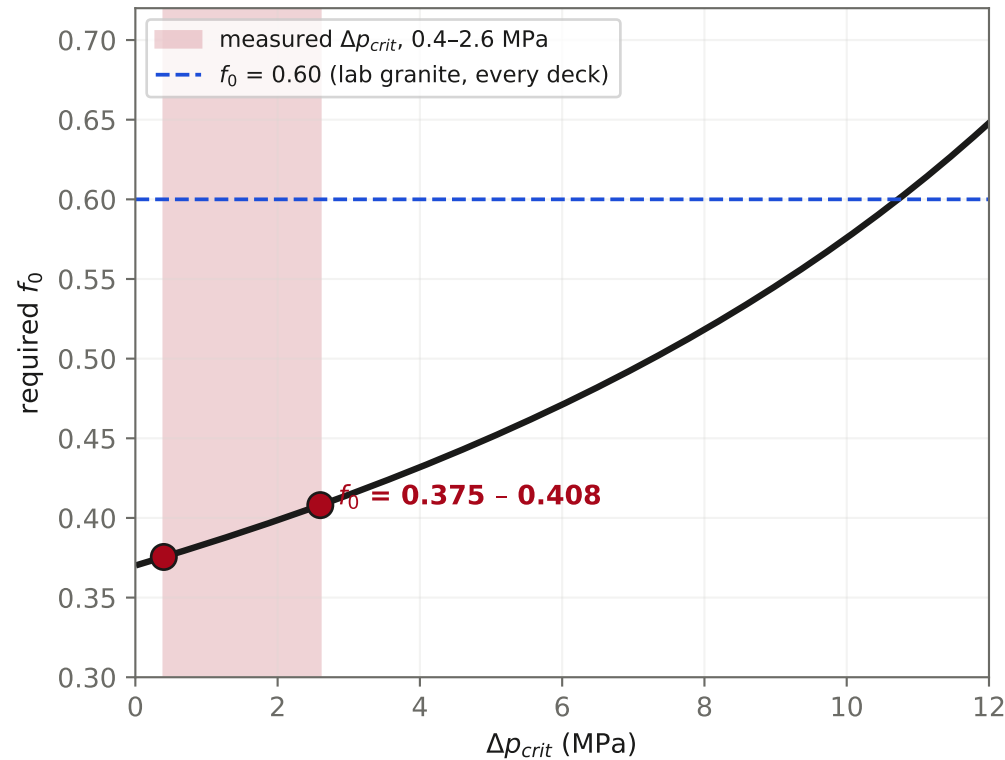
B. f_0 implied by the measurement, at the MEASURED \tau_0 and \bar{\sigma}_0
