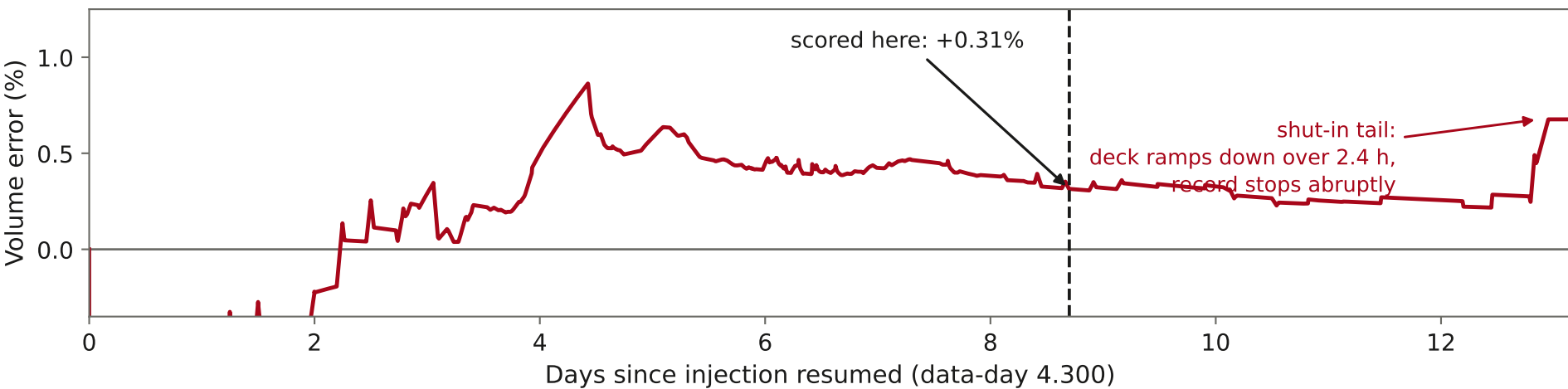
(c) Volume error — deck relative to measured, cumulative to each time
