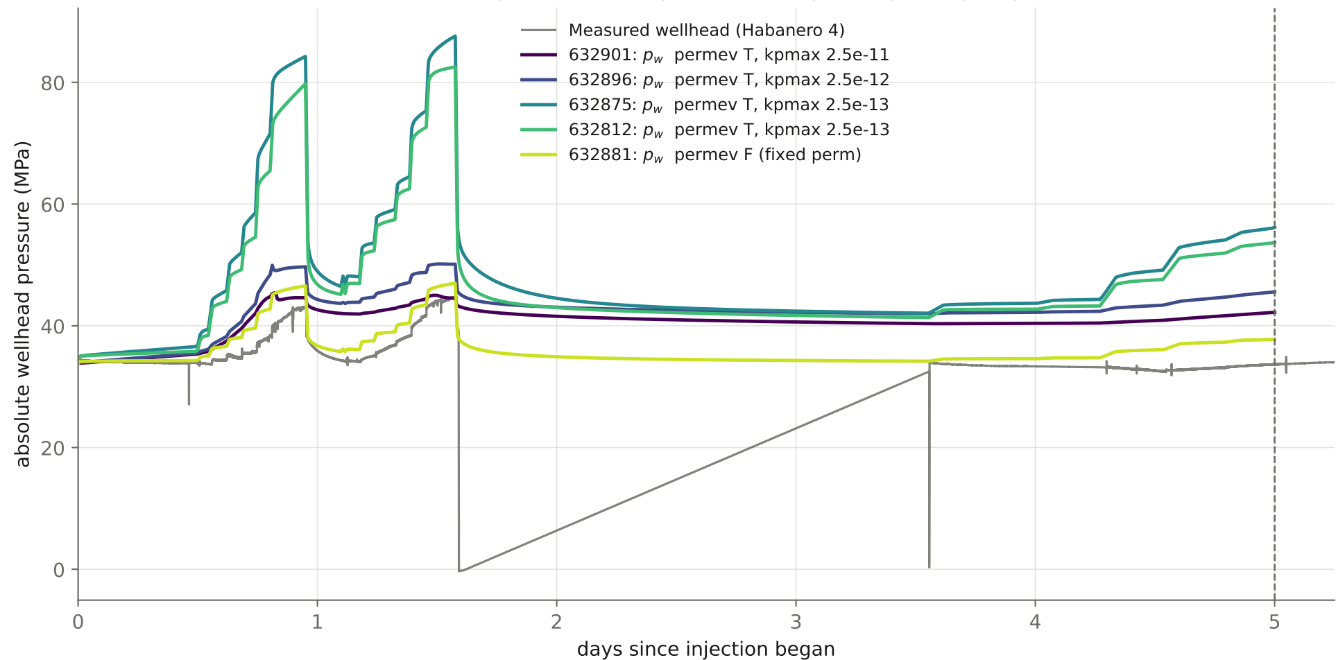
Wellhead pressure: new p_w vs the old p_f -at-injector proxy
