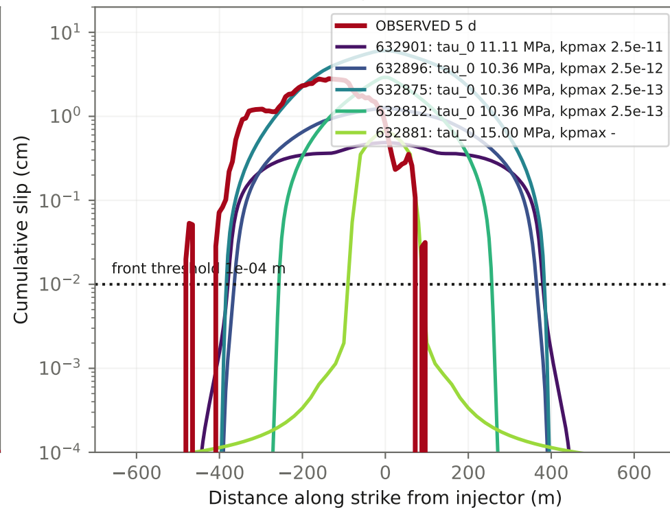
B. Front — where each profile crosses the threshold
