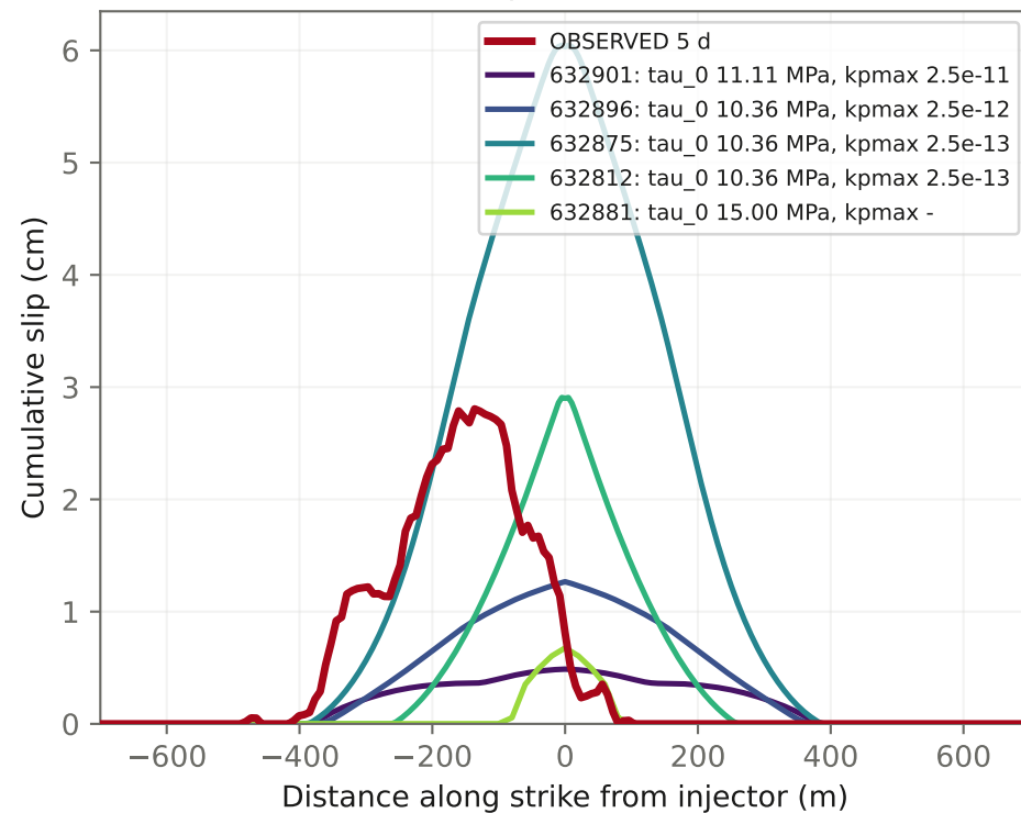
A. Amplitude at 5 d
