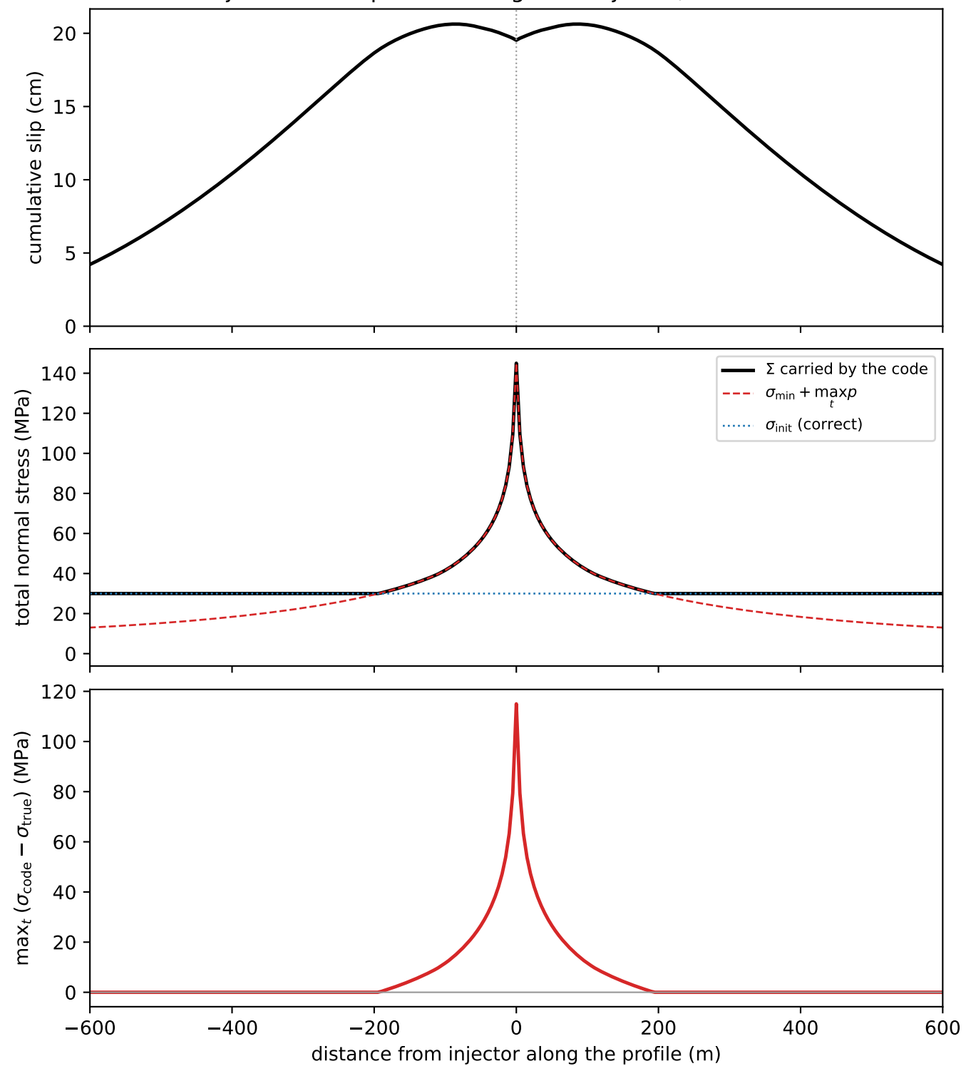
job 632510: profile through the injector, final state
