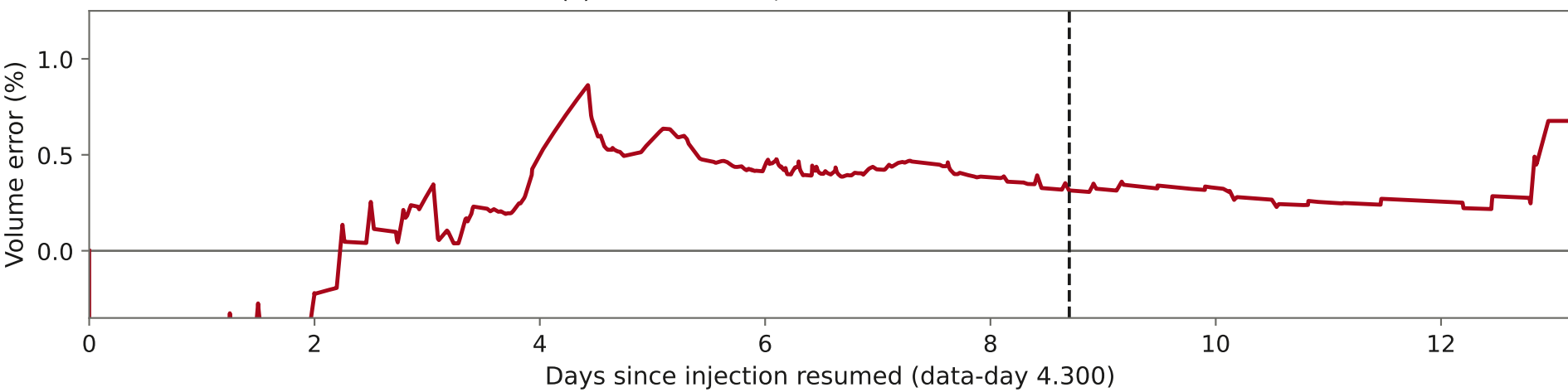
(c) Volume error, file relative to measured
