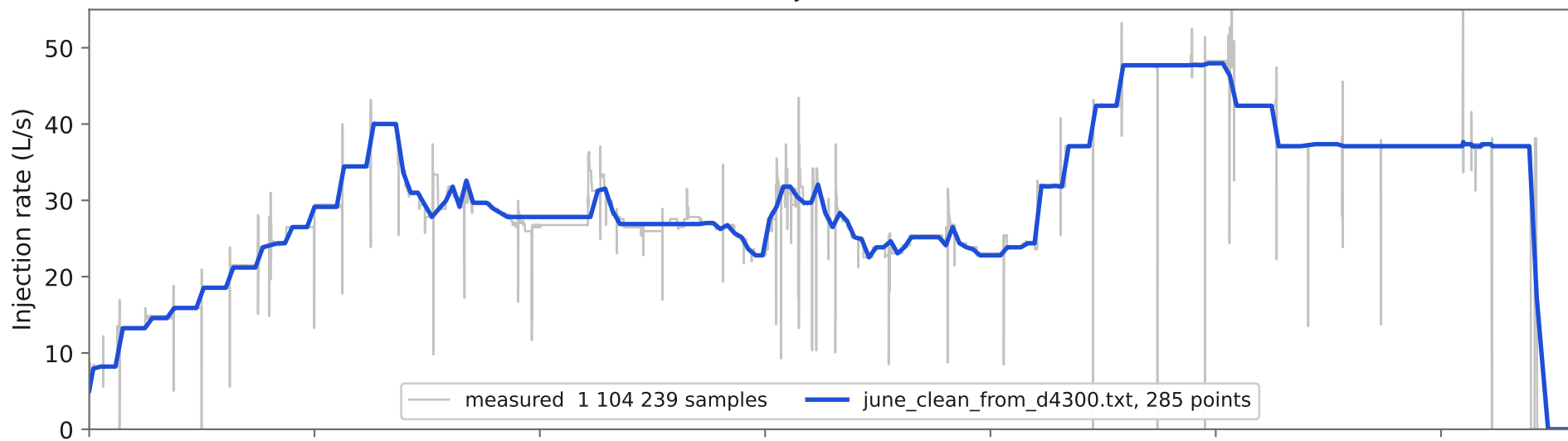
(a) Injection rate
