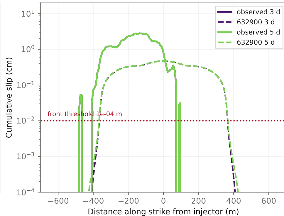
B. Front — the threshold crossings nearly coincide
