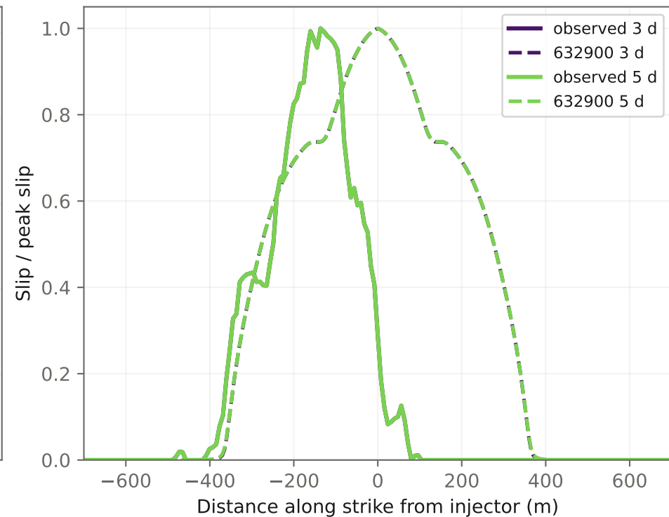
C. Shape — each profile over its own peak
