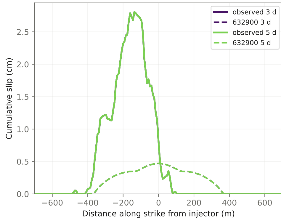
A. Amplitude — solid observed, dashed simulated
