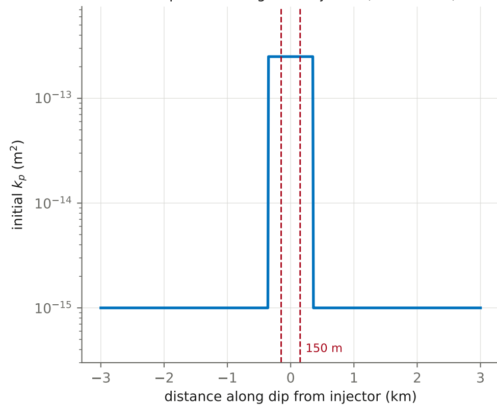
radial profile through the injector (full domain)
