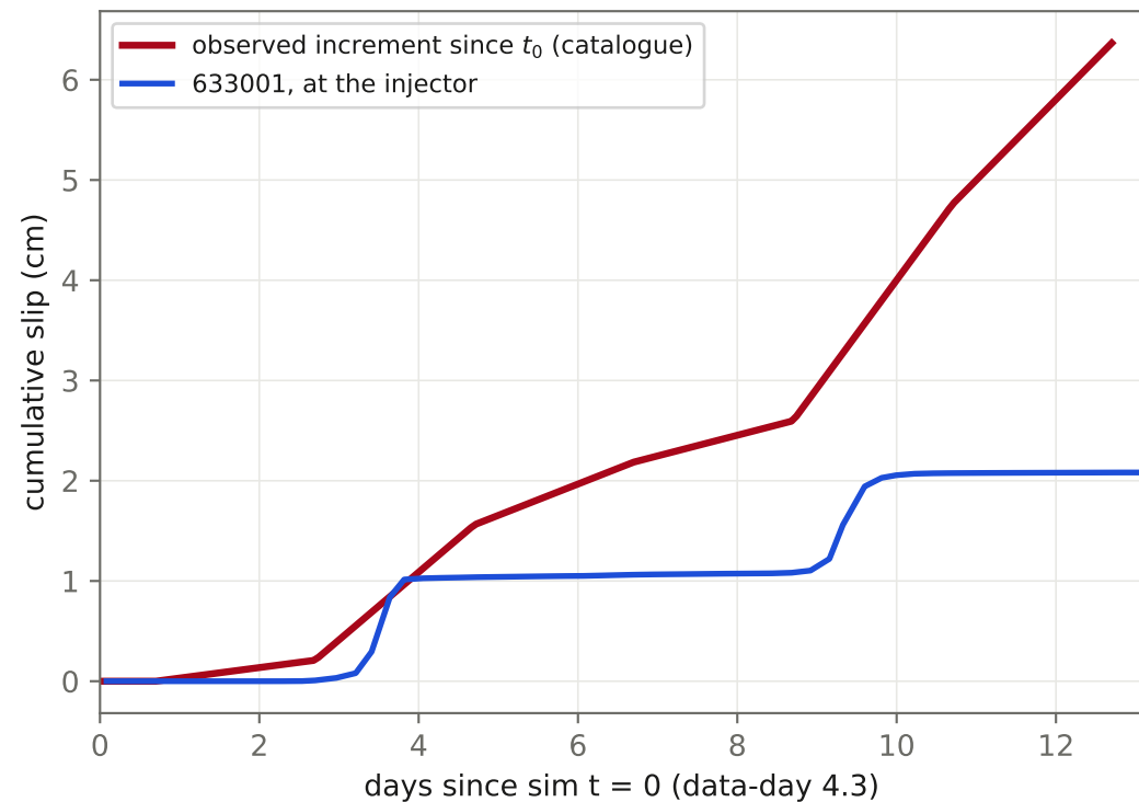
(a) At the injector | 0.42× observed at 8.7 d
