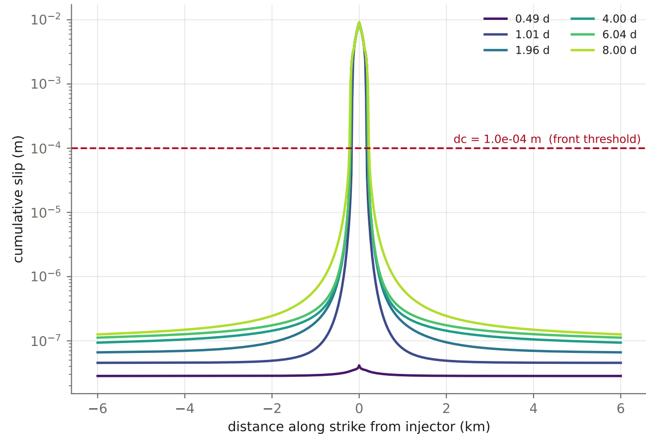
Slip profile along strike (through the injector)
