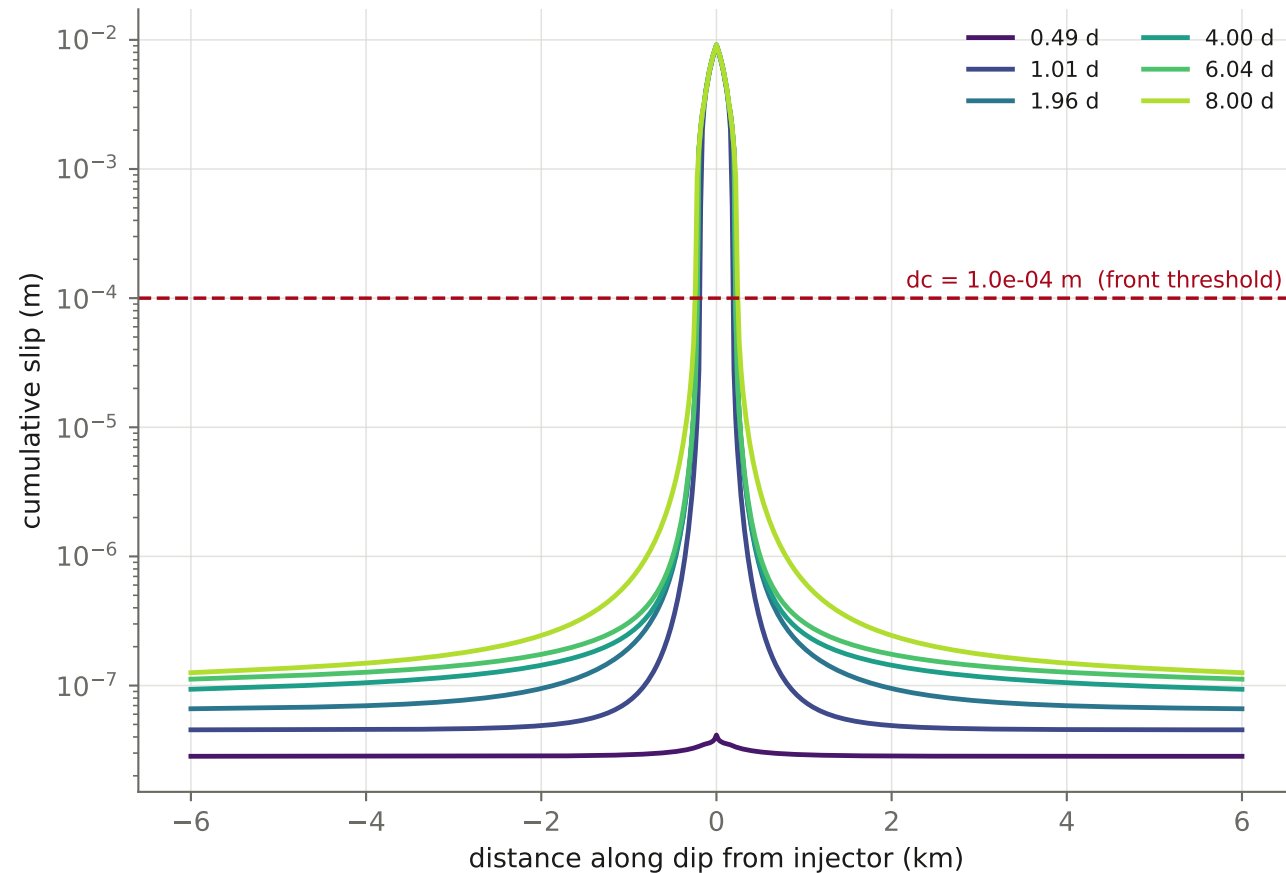
Slip profile along dip (through the injector)
