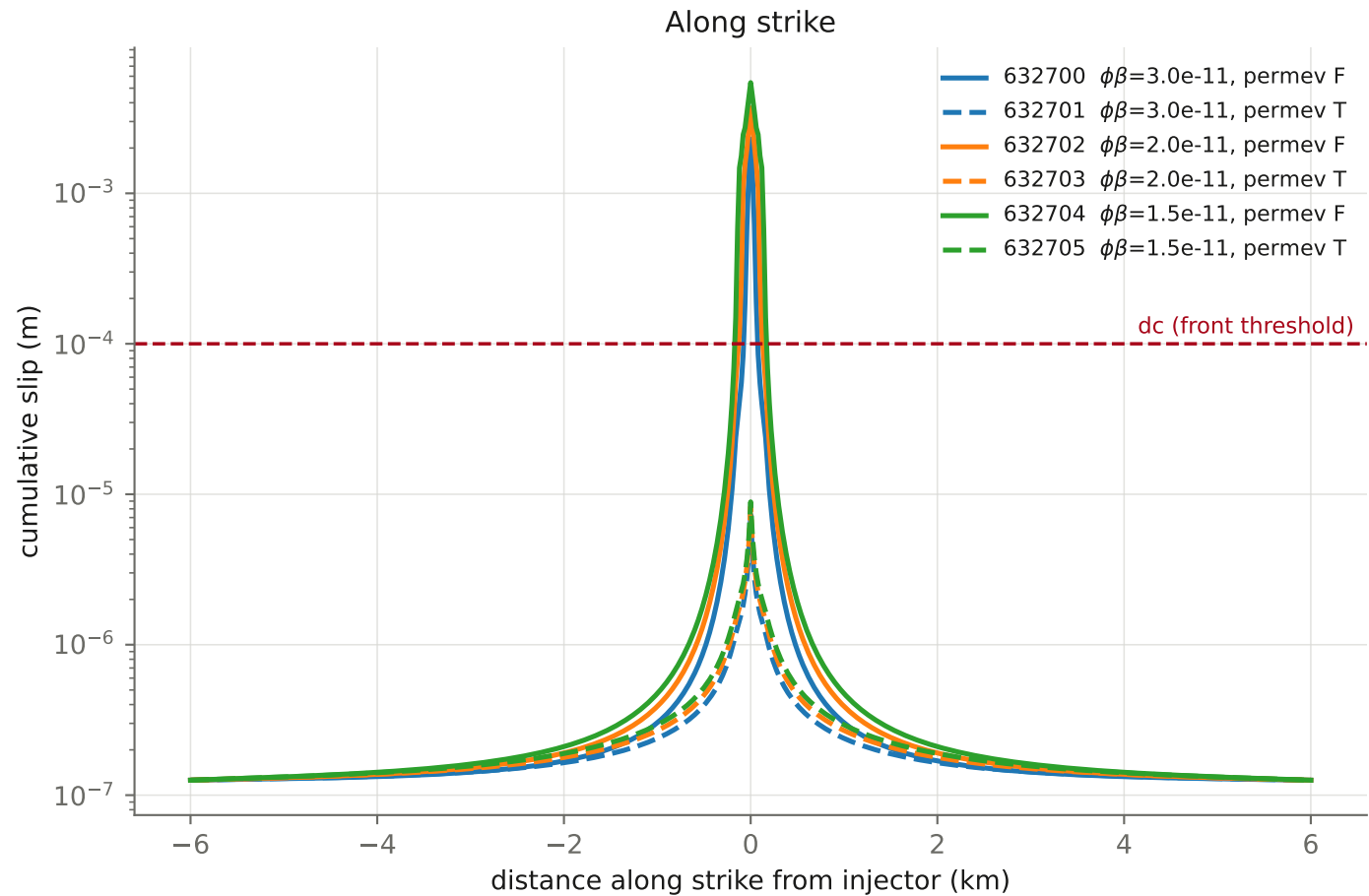
Slip distribution — Effect of permeability enhancement (permev T vs F), matched pairs fixed within each pair: \mu_0=0.46 , \bar{\sigma}_0=27.99 MPa, Taiyi perm map; permev T uses k_{pmax}=2e-11 , k_L=1e-5 all profiles at the shared time 8.00 d
