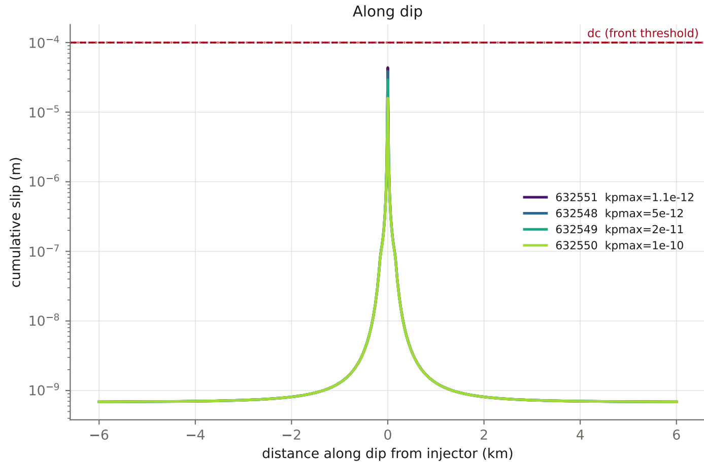
Slip distribution — Effect of enhanced permeability ceiling k_{pmax} fixed: \mu_0=0.37 , \bar{\sigma}_0=27.99 MPa, \phi\beta=1e-10 , permev T, kL=1e-3 , Taiyi perm map all profiles at the shared time 17.20 d
