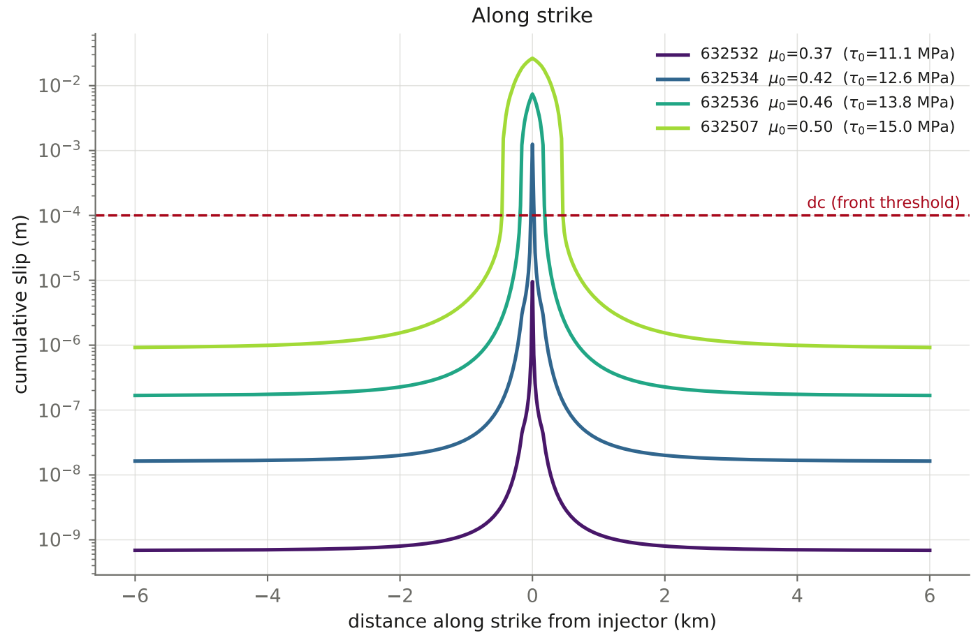
Slip distribution — Effect of initial friction \mu_0 (fault strength) fixed: \bar{\sigma}_0=30.0 MPa, \phi\beta=1e-10 , permev F, Taiyi perm map, dc=1e-4 all profiles at the shared time 17.20 d
