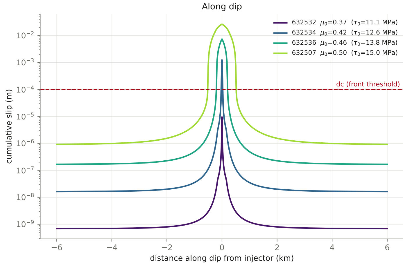
Slip distribution — Effect of initial friction \mu_0 (fault strength) fixed: \bar{\sigma}_0=30.0 MPa, \phi\beta=1e-10 , permev F, Taiyi perm map, dc=1e-4 all profiles at the shared time 17.20 d
