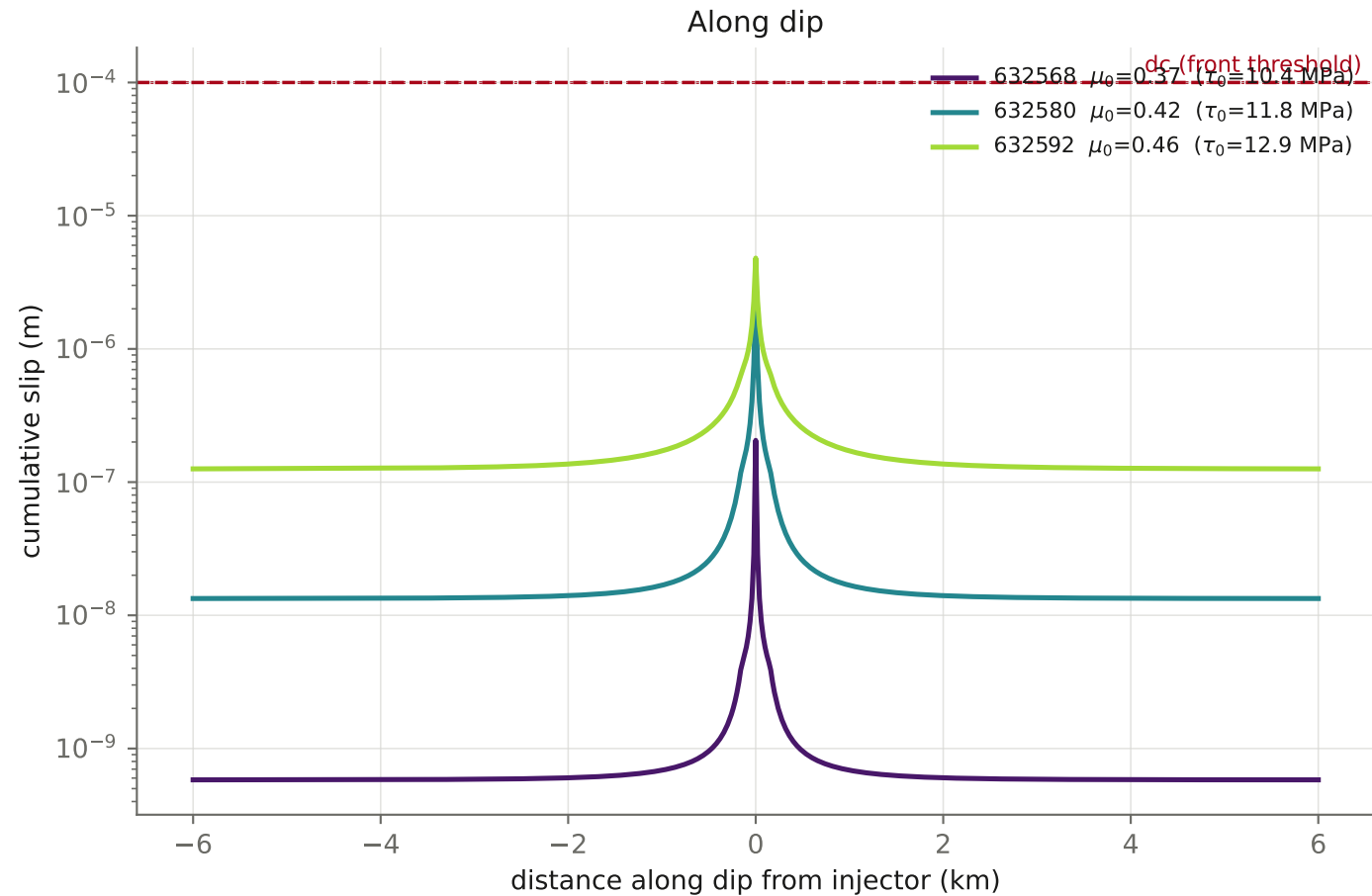
Slip distribution — Effect of \mu_0 with permeability enhancement ON fixed: \bar{\sigma}_0=27.99 MPa, \phi\beta=1e-10 , permev T, kpmx=2e-11, kpmn=4e-13, kL=1e-5, Taiyi perm map, dc=1e-4 all profiles at the shared time 8.00 d
