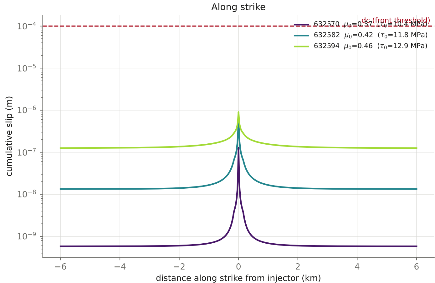
Slip distribution — Effect of \mu_0 with enhancement ON at the highest defensible k p max fixed: \bar{\sigma}_0=27.99 MPa, \phi\beta=1e-10 , permev T, k p max=1e-10 ( \approx 100 D), k p min=4e-13, k L =1e-5, Taiyi perm map all profiles at the shared time 8.00 d
