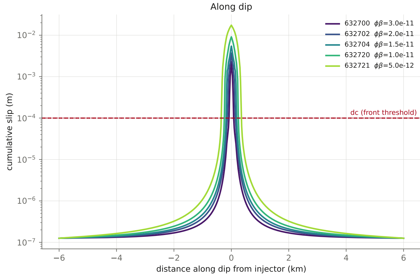
Slip distribution — Effect of storage \phi\beta at understressed \mu_0=0.46 fixed: \mu_0=0.46 , \bar{\sigma}_0=27.99 MPa ( \tau_0=12.9 MPa, understressed), permev F, Taiyi perm map all profiles at the shared time 8.00 d
