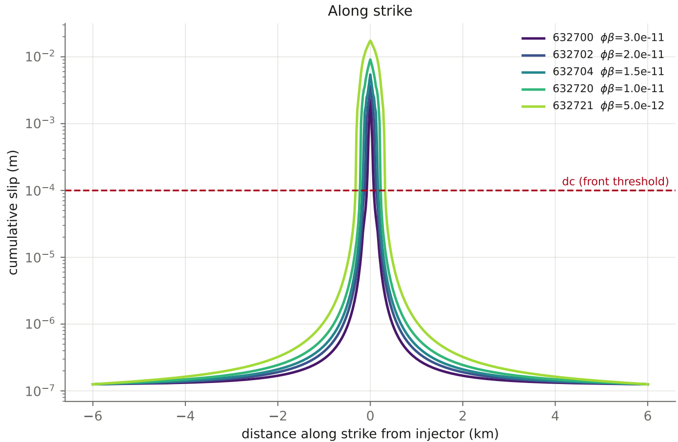
Slip distribution — Effect of storage \phi\beta at understressed \mu_0=0.46 fixed: \mu_0=0.46 , \bar{\sigma}_0=27.99 MPa ( \tau_0=12.9 MPa, understressed), permev F, Taiyi perm map all profiles at the shared time 8.00 d
