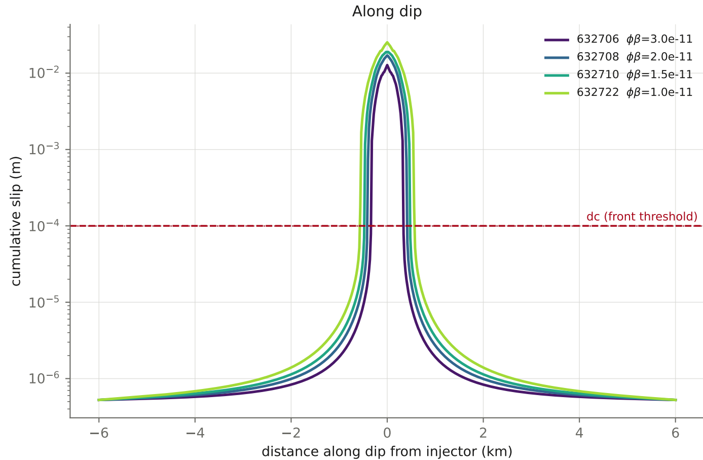
Slip distribution — Effect of storage \phi\beta at \mu_0=0.50 (Taiyi-equivalent stress) fixed: \mu_0=0.50 , \bar{\sigma}_0=27.99 MPa, permev F, Taiyi perm map all profiles at the shared time 8.00 d
