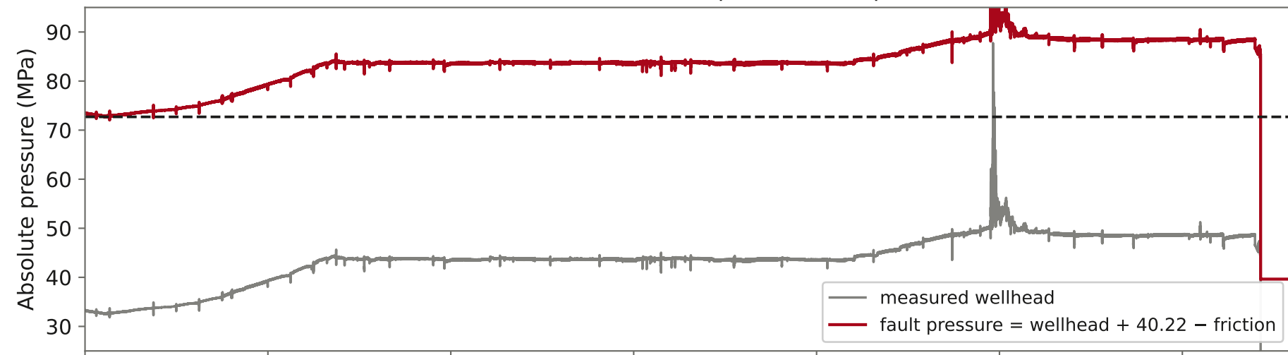
(a) Measured wellhead, and the fault pressure it implies at \rho = 1000
