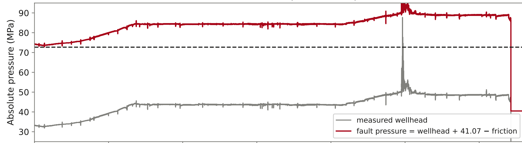
(a) Measured wellhead, and the fault pressure it implies at \rho = 1001
