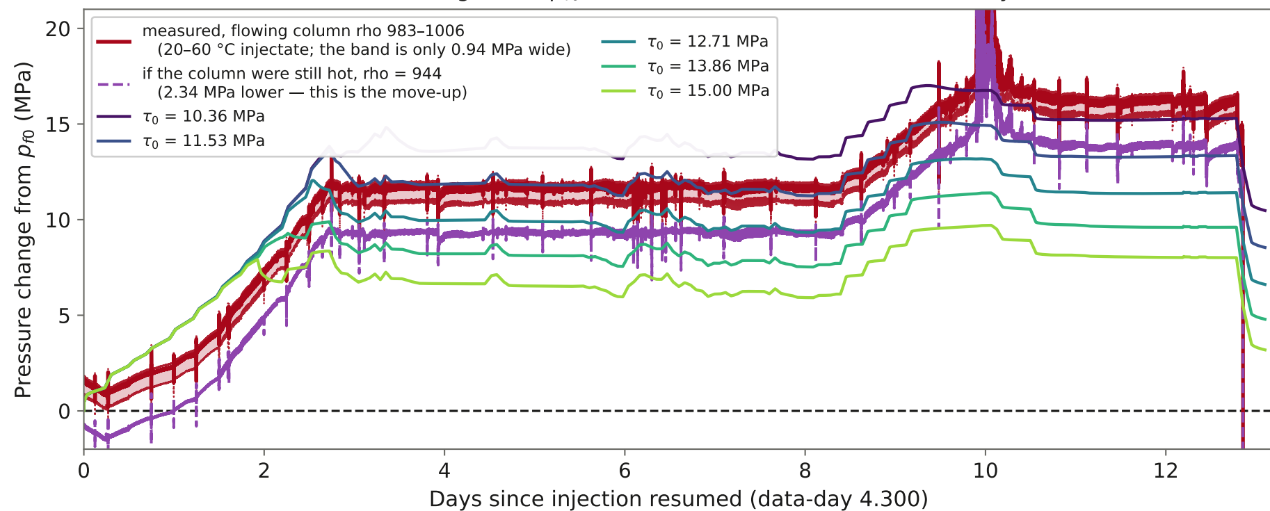
(b) Pressure change from p_{f0} = 72.70 MPa, with the column-density bracket
