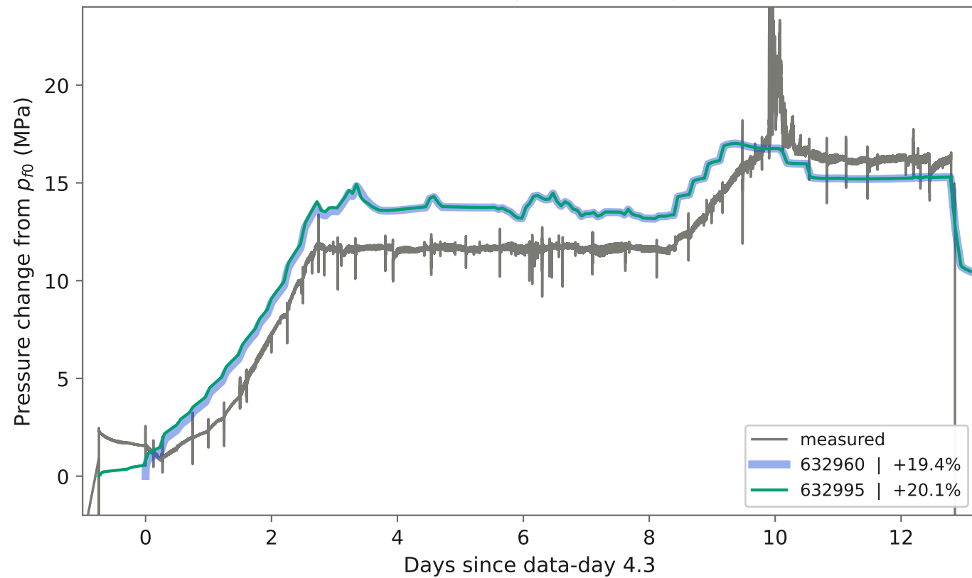
(c) Wellhead pressure change
