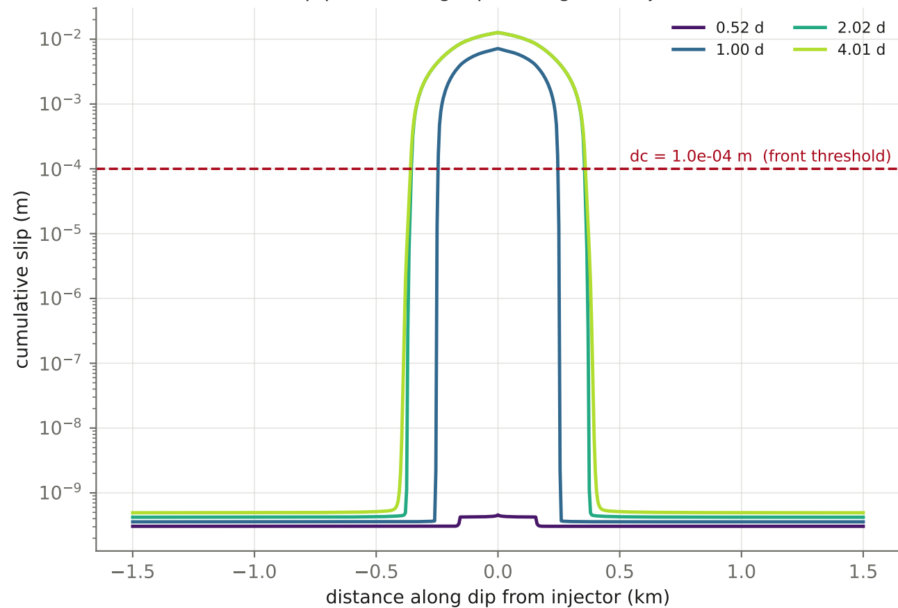
Slip profile along dip (through the injector)
