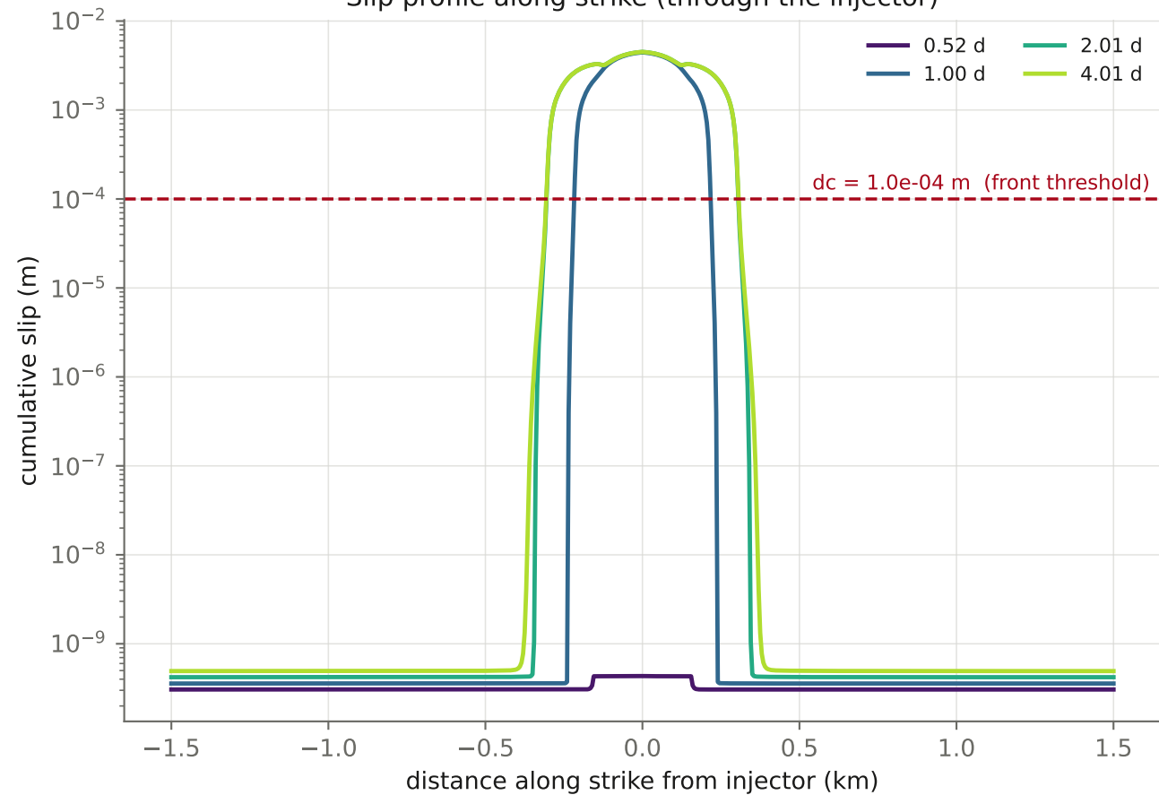
Slip profile along strike (through the injector)
