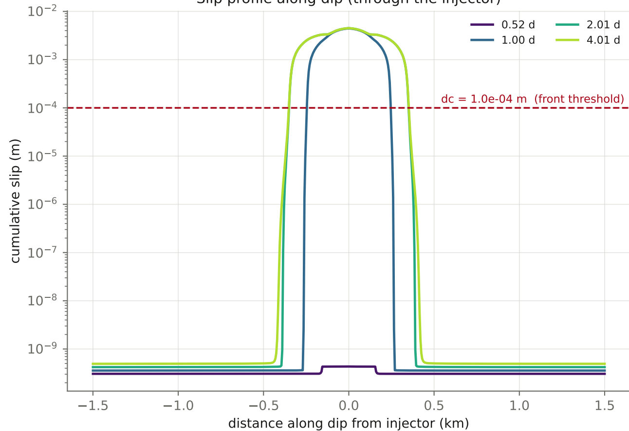
Slip profile along dip (through the injector)
