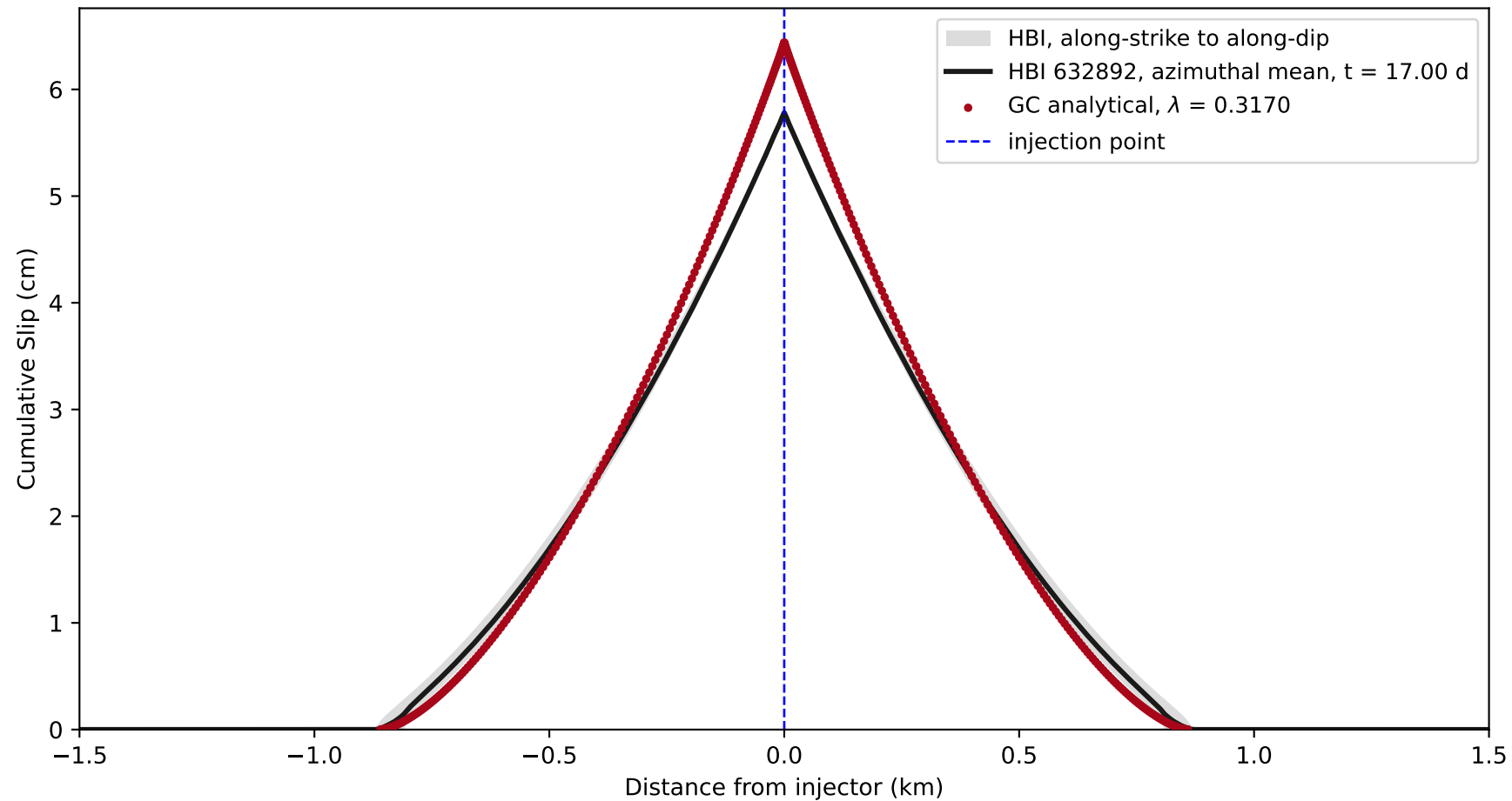
GC analytical solution vs HBI 632892 at t = 17 days T = 9.583 , \lambda = 0.3170 , R_t = 859 m, \alpha = 1.25 , \Delta P = 1.2 MPa
