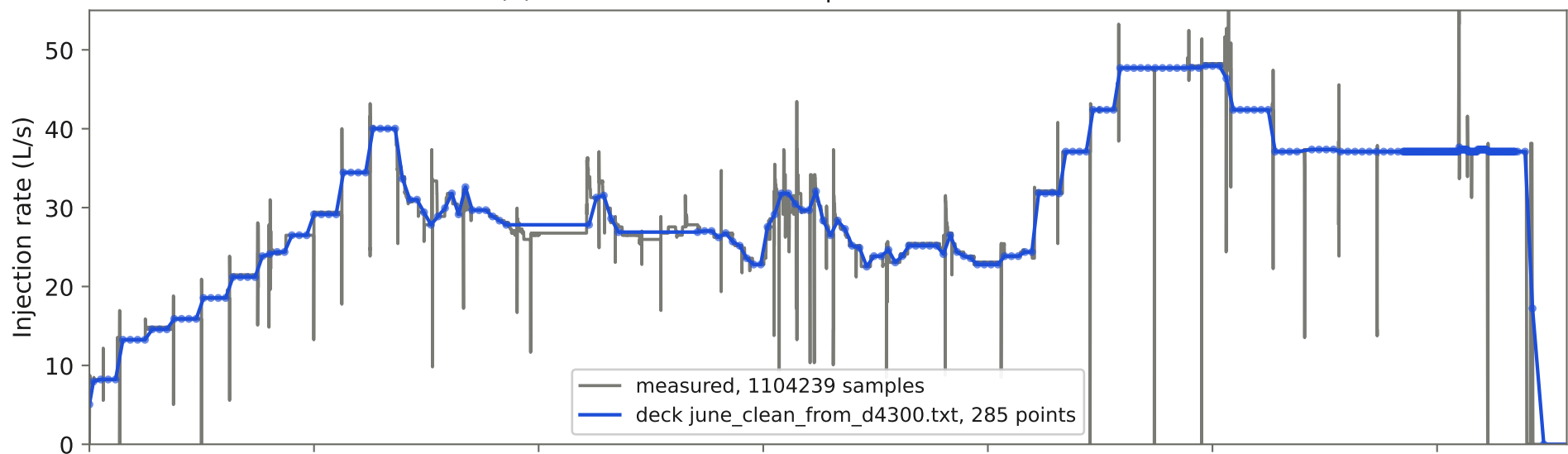
(a) Rate — does the 285-point file follow the record
