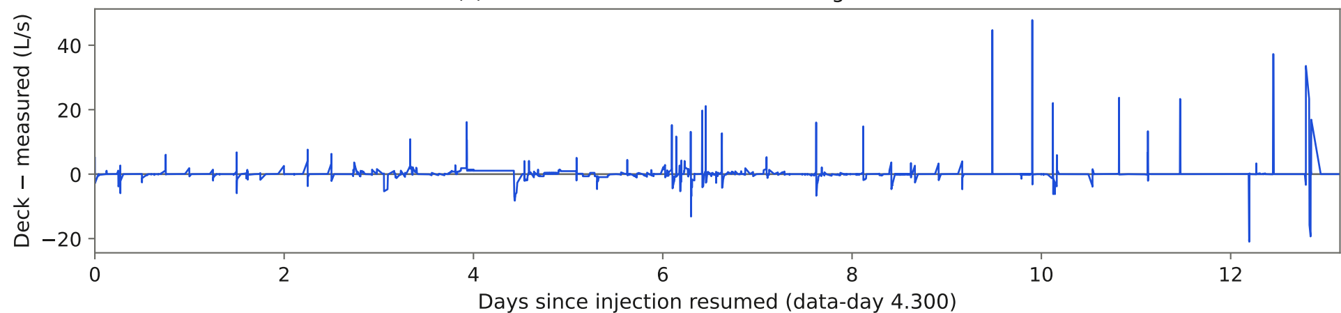
(c) Rate residual — where the disagreement sits
