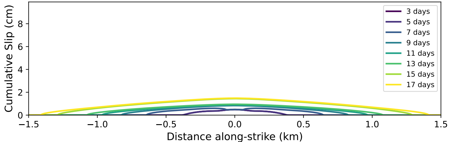
Job 632910: \tau_0 = 11.11 MPa, k_{pmax} 2.5e-11
