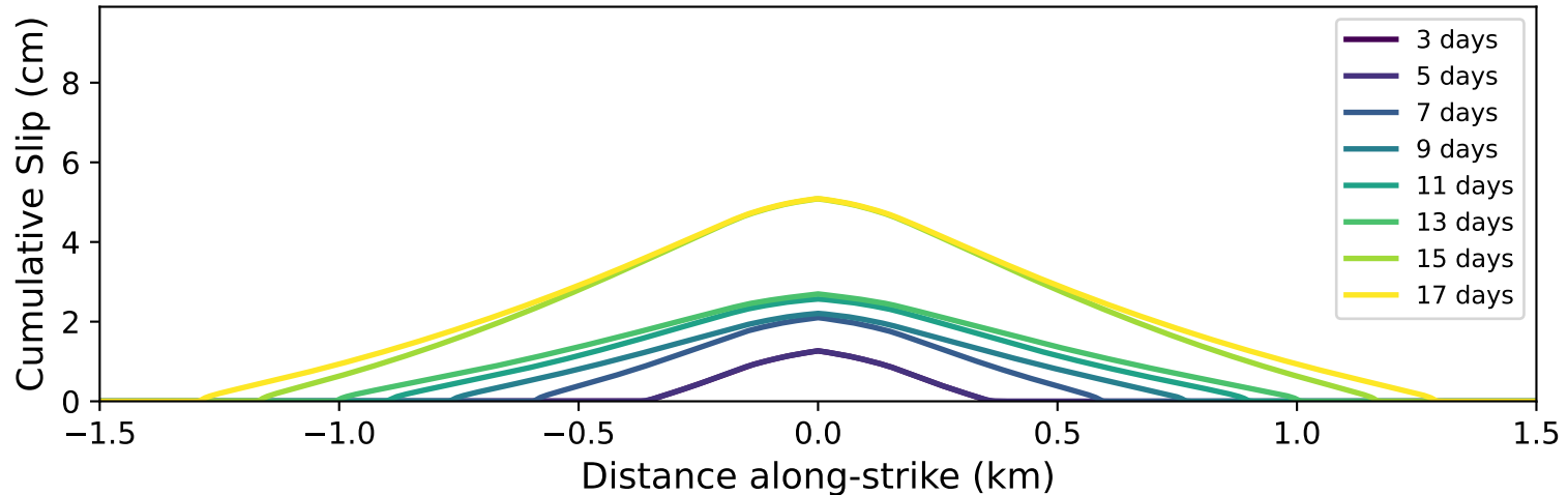
Job 632911: \tau_0 = 10.36 MPa, k_{pmax} 2.5e-12
