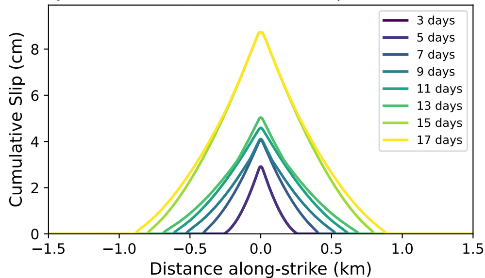
Job 632916: \tau_0 = 11.11 MPa, k_{pmax} 2.5e-11
