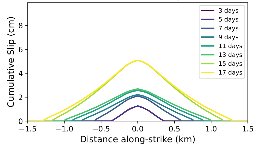
Job 632917: \tau_0 = 11.11 MPa, k_{pmax} 2.5e-11
