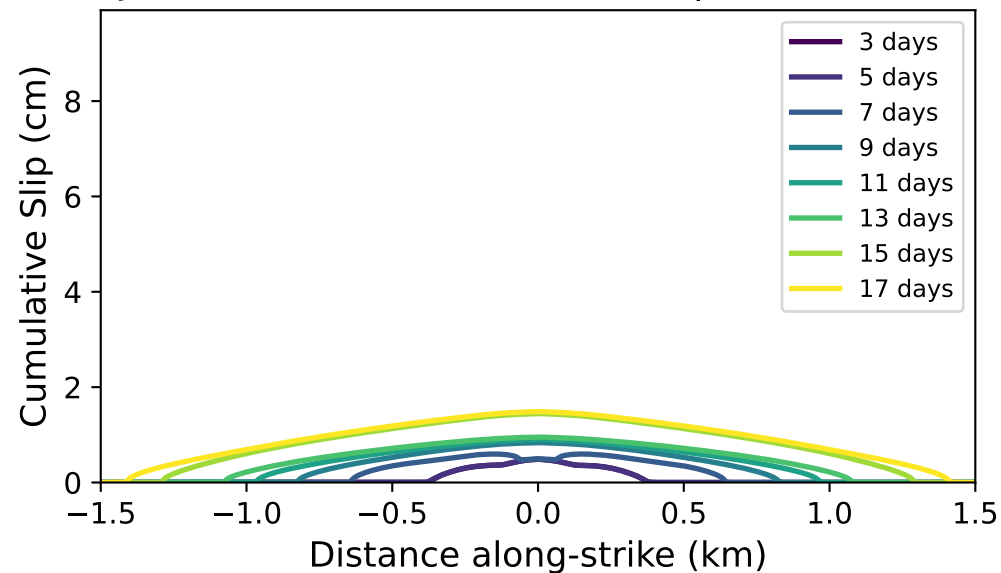
Job 632910: \tau_0 = 11.11 MPa, k_{pmax} 2.5e-11
