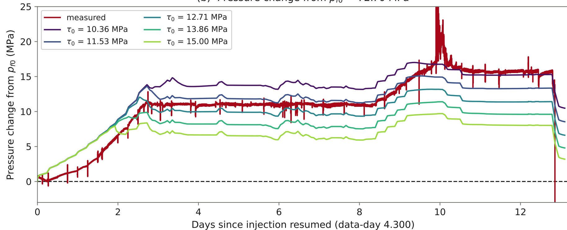
(b) Pressure change from p_{f0} = 72.70 MPa
