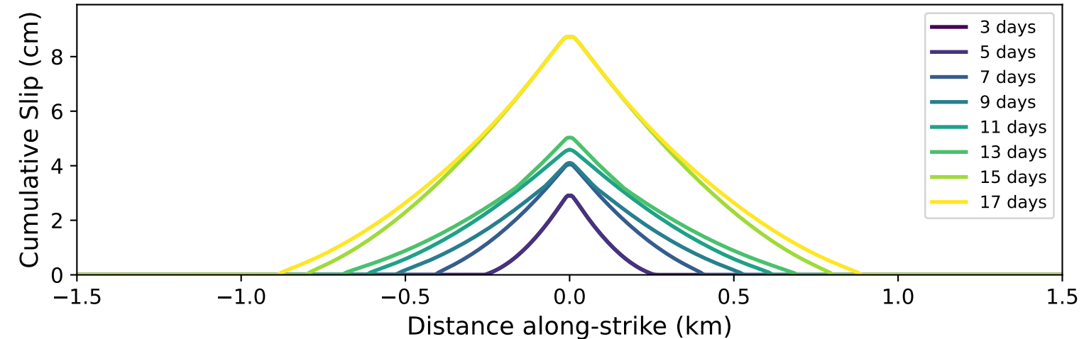
Job 632913: \tau_0 = 10.36 MPa, k_{pmax} 2.5e-13
