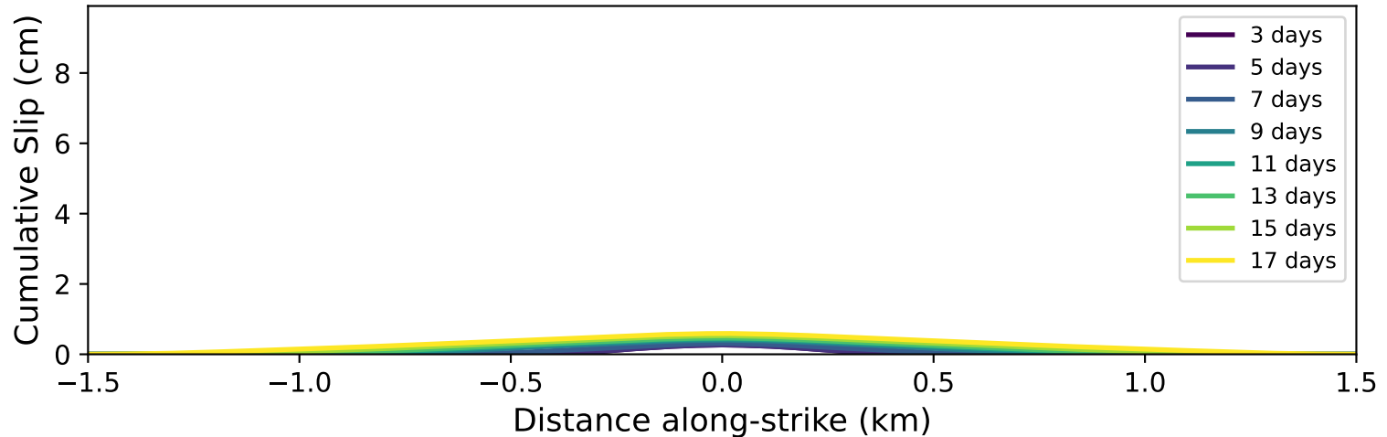
Job 632915: \tau_0 = 11.11 MPa, k_{pmax} 2.5e-11
