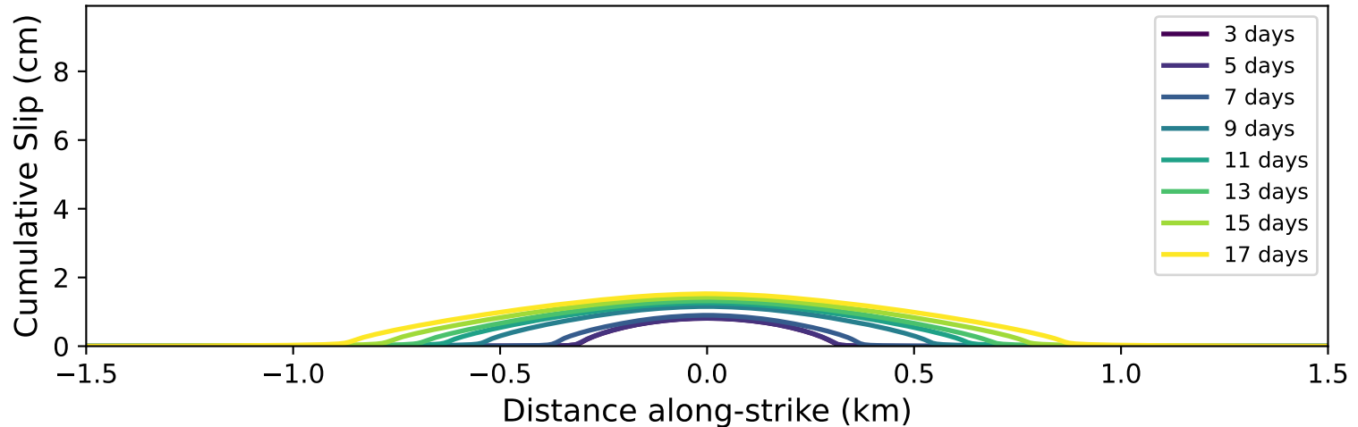
Job 632916: \tau_0 = 11.11 MPa, k_{pmax} 2.5e-11
