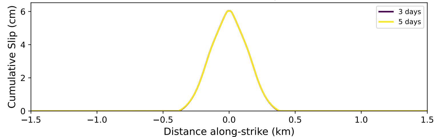
Job 632875: \tau_0 = 10.36 MPa, k_{pmax} 2.5e-13
