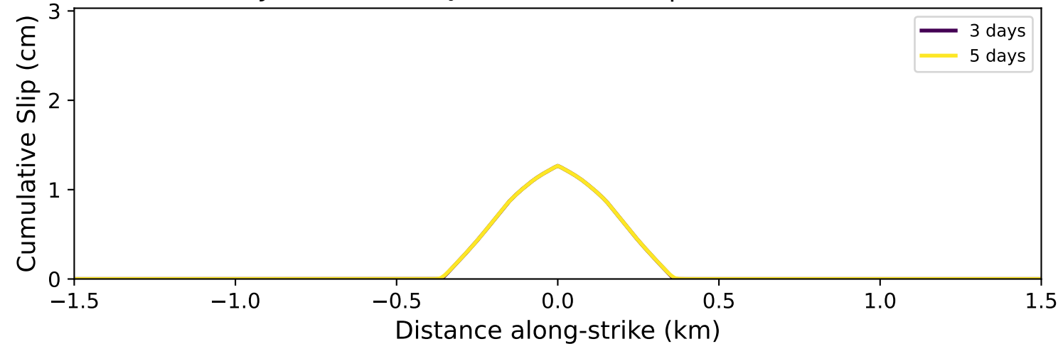
Job 632896: \tau_0 = 10.36 MPa, k_{pmax} 2.5e-12
