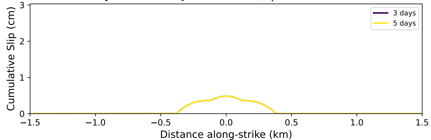
Job 632901: \tau_0 = 11.11 MPa, k_{pmax} 2.5e-11
